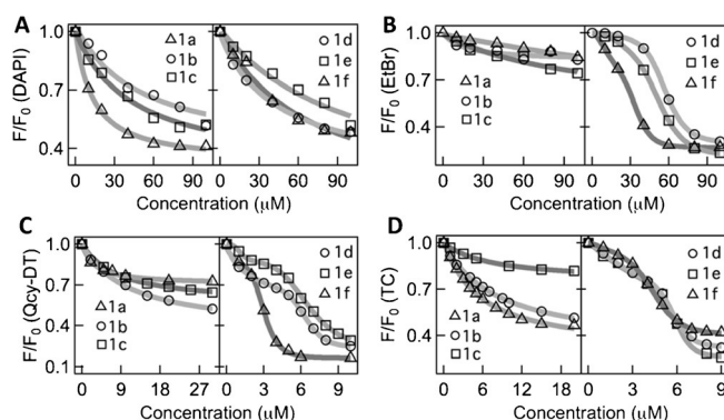
Figure 4. Fluorescence quenching of 10 \mu\text{M} ct-DNA and 10 \mu\text{M} DAPI ( \lambda_{\text{ex}} = 338\text{ nm} ; A), 20 \mu\text{M} ct-DNA and 10 \mu\text{M} EtBr ( \lambda_{\text{ex}} = 480\text{ nm} ; B), 10 \mu\text{M} ct-DNA and 2 \mu\text{M} Qcy-DT ( \lambda_{\text{ex}} = 564\text{ nm} ; C), and 10 \mu\text{M} ct-DNA and 10 \mu\text{M} TC ( \lambda_{\text{ex}} = 521\text{ nm} ; D) by compounds 1a-f (in buffer A at 25 ^{\circ}\text{C} ). The solid lines are the best fits to the data using a Langmuir isotherm (A, and the left panels of B, C, and D) or a sequential model (the right panels of B, C, and D). Maximum error along the abscissa is 0.1 units (all fluorescence spectra were corrected for inner filter effect).
